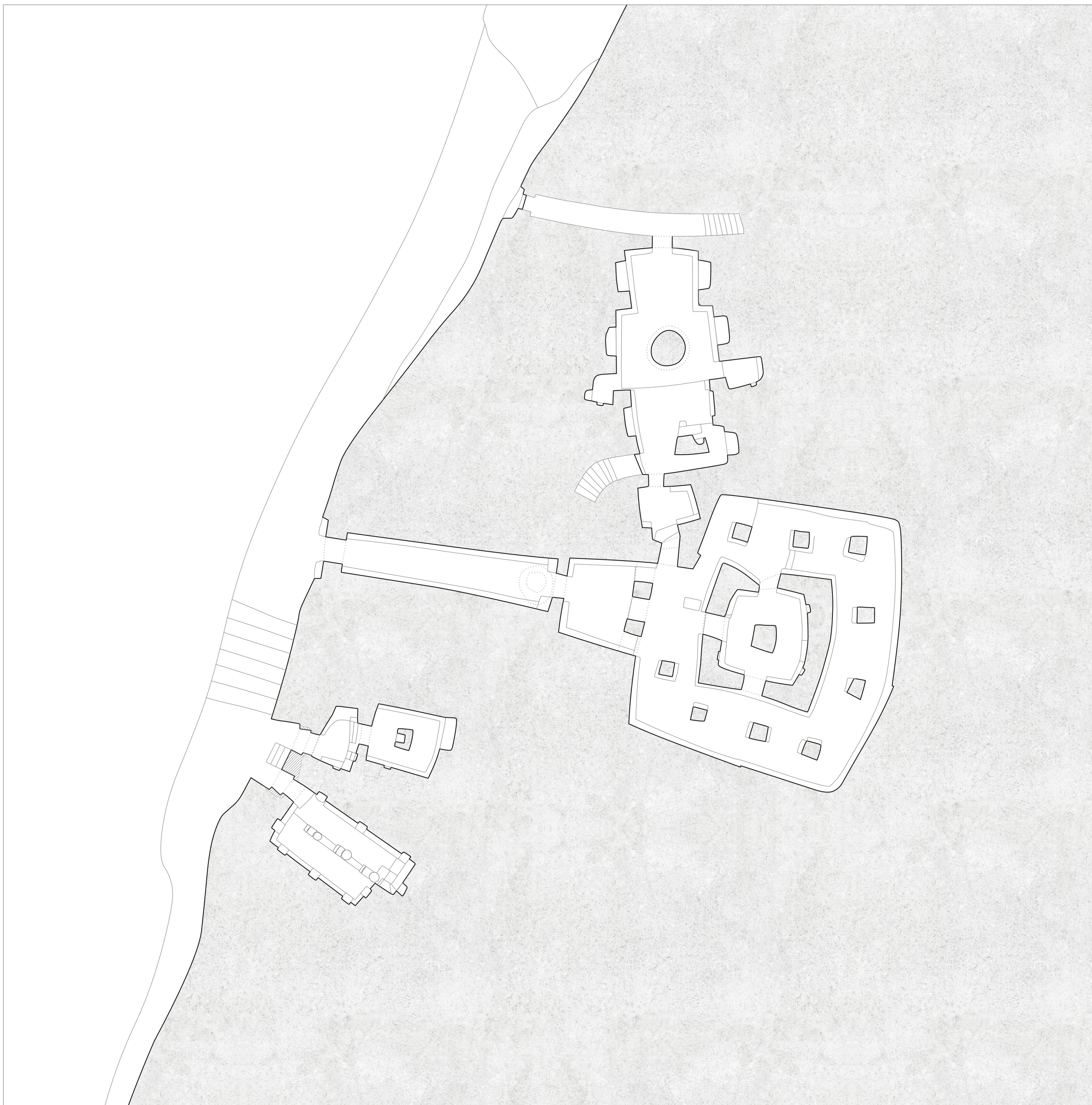
Gologtha (Lower Complex), Ground Floor Plan (2018)
