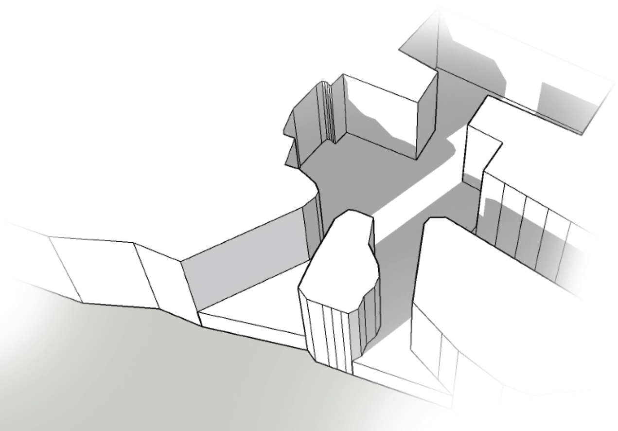
Axonometric layout of the excavation
